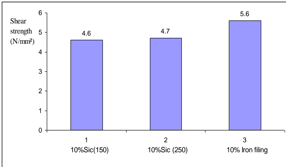
Figure (4): Comparison between the addition of (10% Sic) particles and (10%) iron filing on shear strength of galvanized (steel / steel) specimens.
