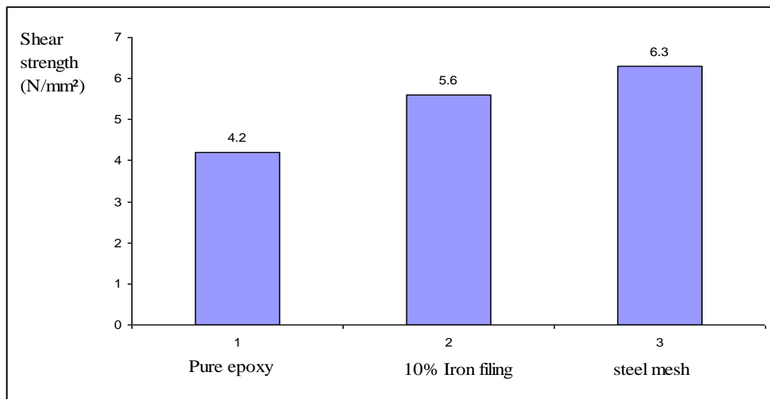
Figure (6): Comparison between the best results of adhesion steel / steel specimens
