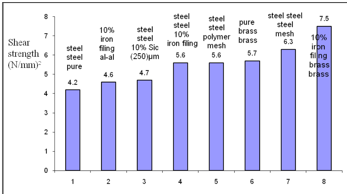
Figure (11): comparison between the shear strength of different types of the experimental results
