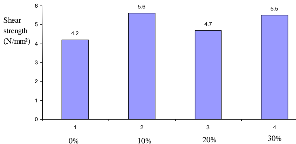
Figure (3): Effect of iron filing percentage on the shear strength of galvanized (steel / steel) specimens.
