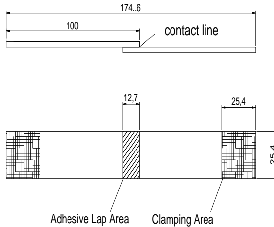
Figure (1): standard single lap joint (Dimensions in mm)
