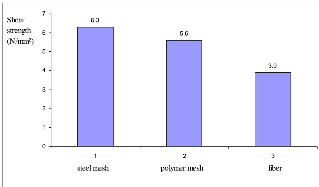
Figure (5): Effect of mesh type added to the epoxy on shear strength of galvanized (steel / steel) specimens.
