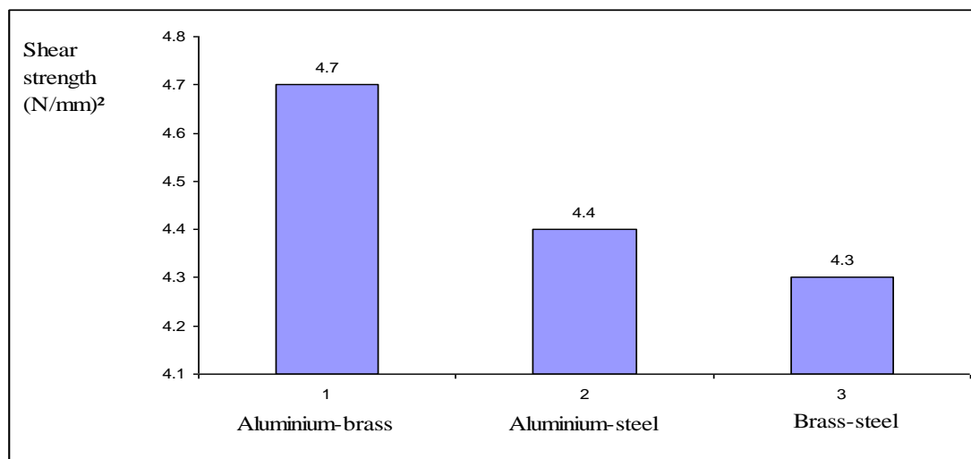
Figure (9): Effect of addition of 10% iron filing on the shear strength of dissimilar metals
