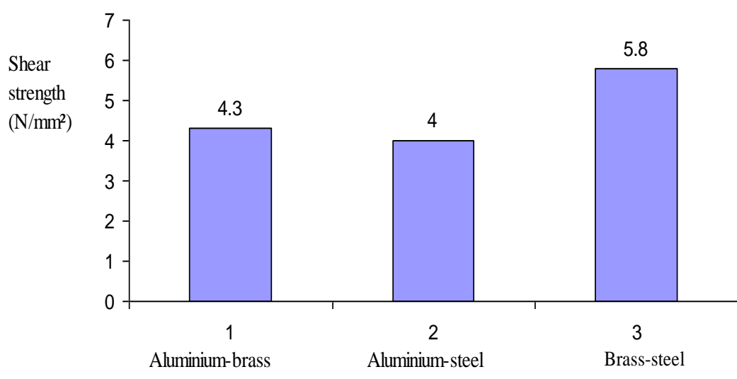
Figure (10): Effect of steel mesh added to the epoxy on the shear strength of dissimilar metals
