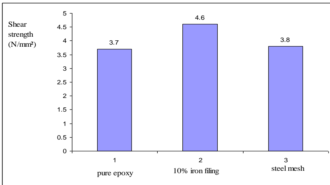
Figure (8): Effect of s reinforcement materials on the shear strength of aluminum/aluminum specimens
