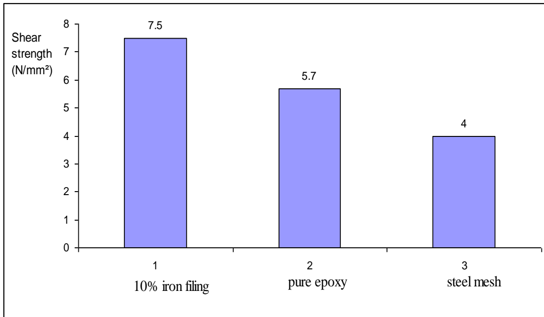
Figure (7): Effect of reinforcement materials on shear strength of brass / brass specimens.
